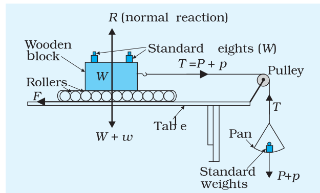
Fig. A 4.1: Setup to study rolling friction
